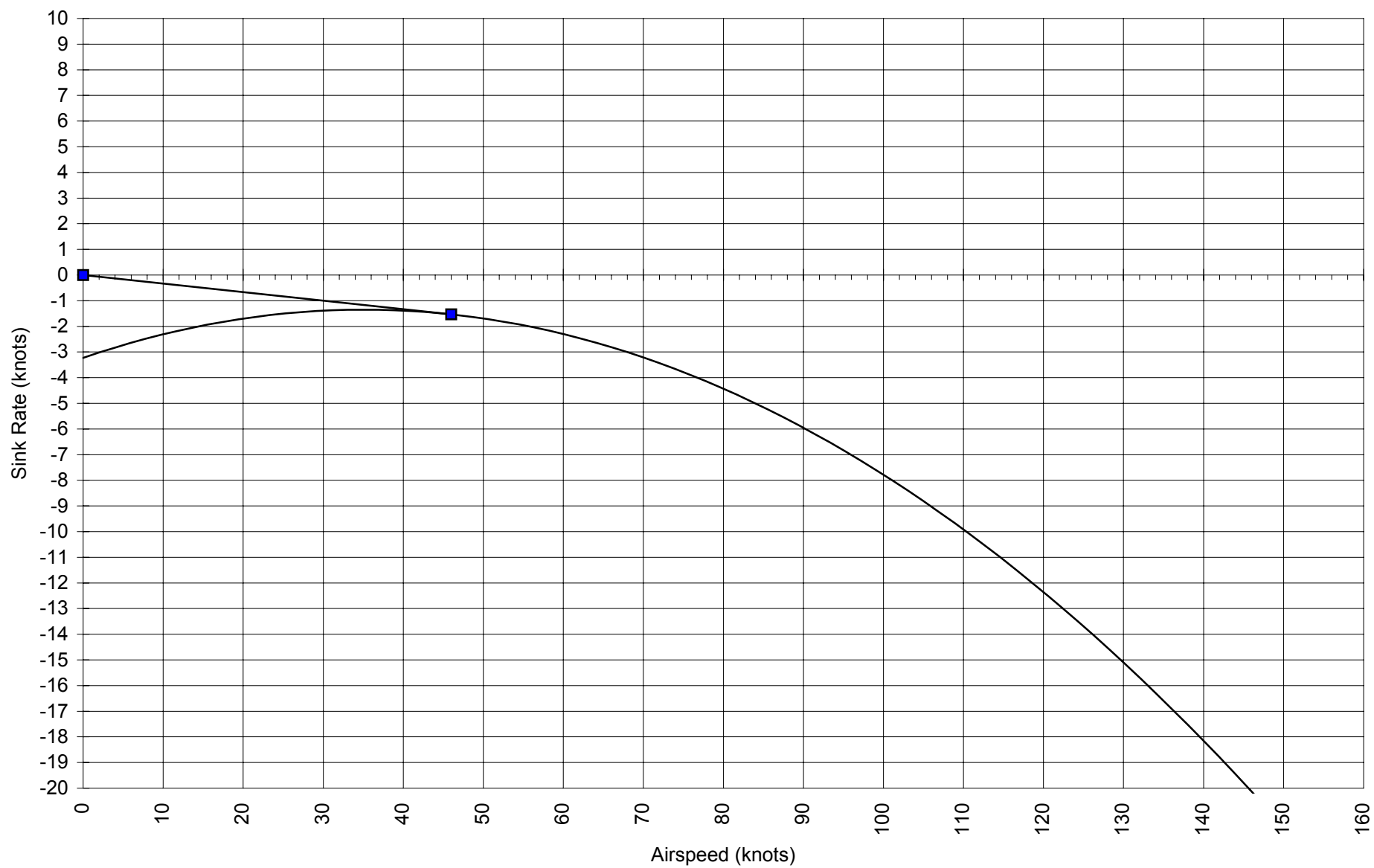
SZD-50-3 Puchacz Polar Plot (2nd order polynomial model) at 1100 lb
