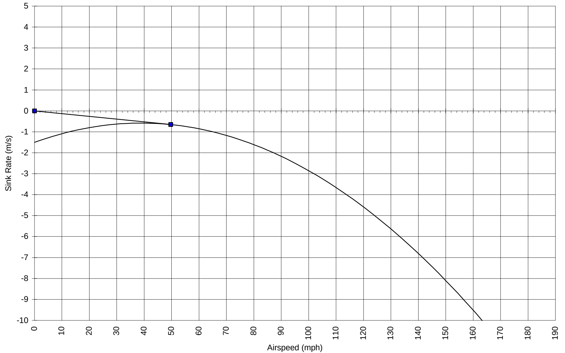
SZD-51-1 Junior Polar Plot (2nd order polynomial model) at 333 kg
