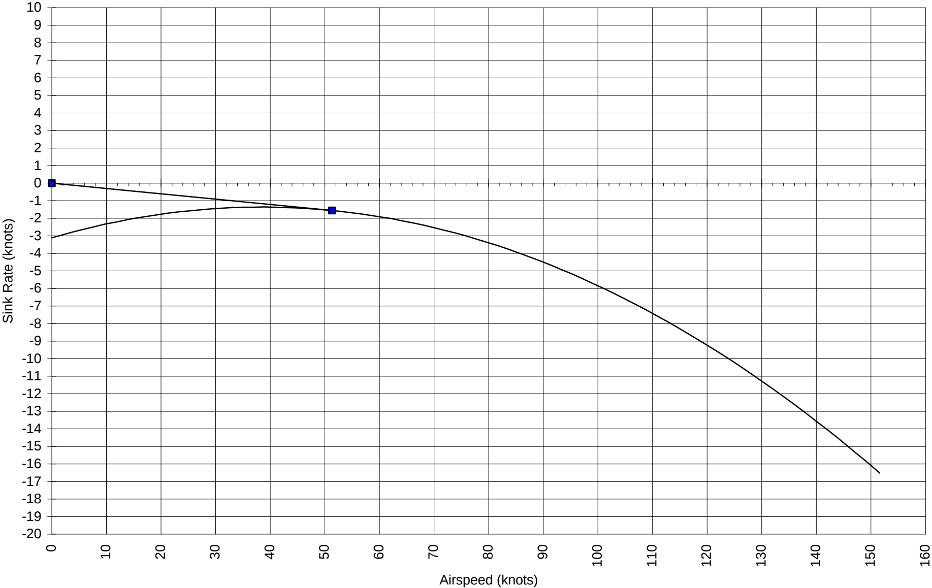
ASK-21 Polar Plot (2nd order polynomial model) at 570 kg
