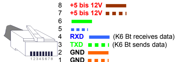
image 3: Pinout of the RJ45 connectors (IGC conform)
