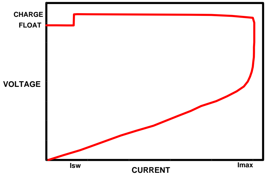
CHARGE CURVE (dual stage)
